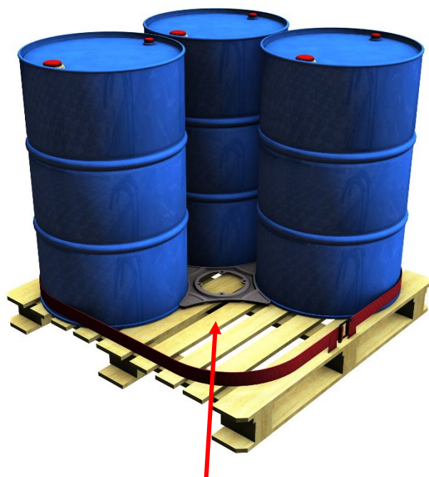
Lasistern® 4, securing four drums on a pallet
